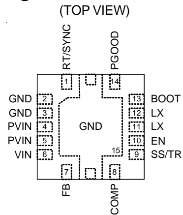
WQFN-14AL 3.5x3.5
